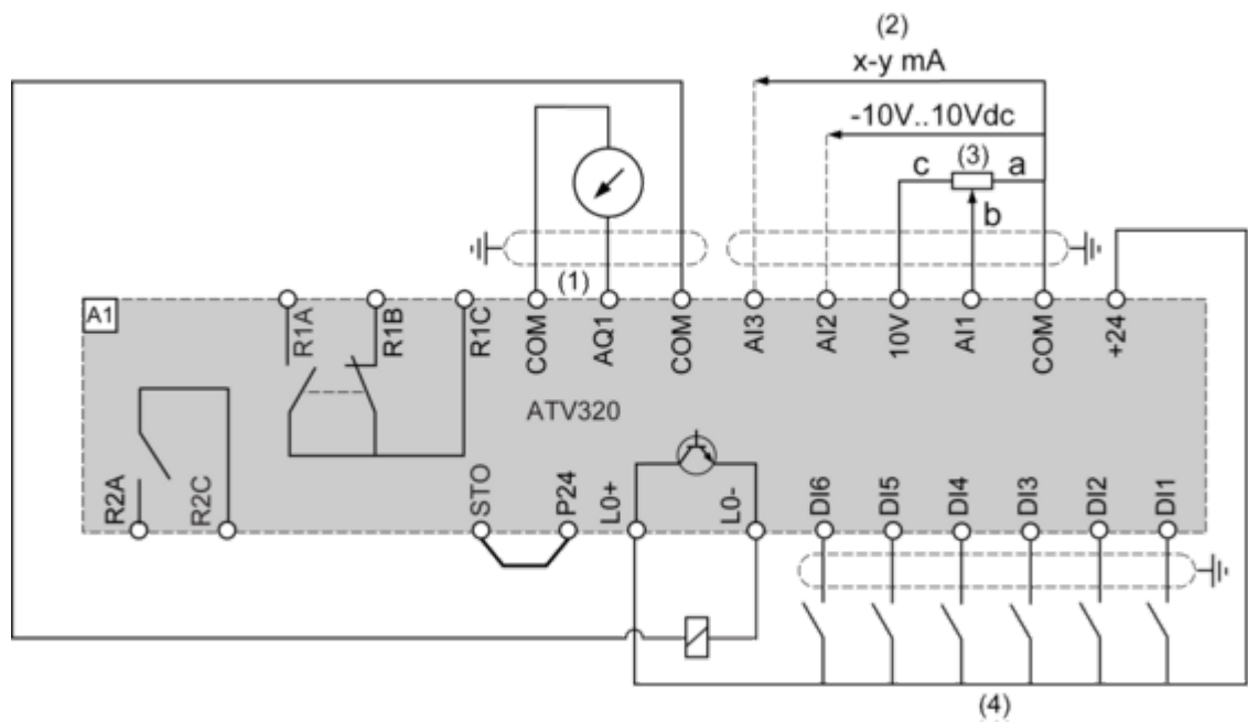
Control Connection Diagram in Source Mode
